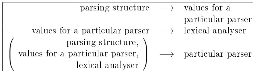
Figure 3: Module Dependencies
